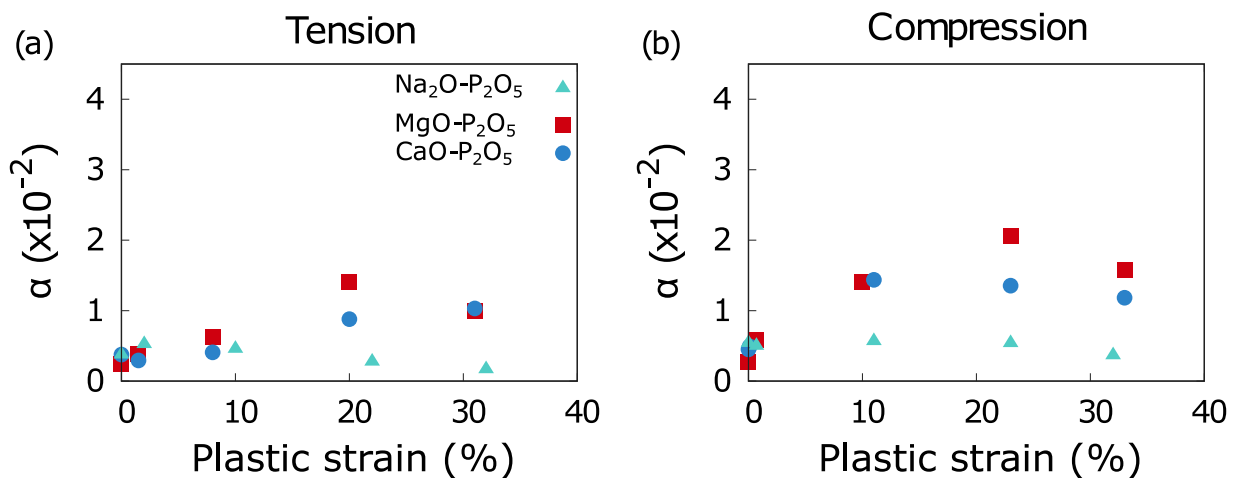
Fig. 3. Anisotropy index as a function of the plastic strain for \text{Na}_2\text{O-P}_2\text{O}_5 , \text{MgO-P}_2\text{O}_5 , and \text{CaO-P}_2\text{O}_5 glasses at 300 K and using a strain rate of 5.0 \times 10^8 \text{ s}^{-1} . (a) tension and (b) compression.
