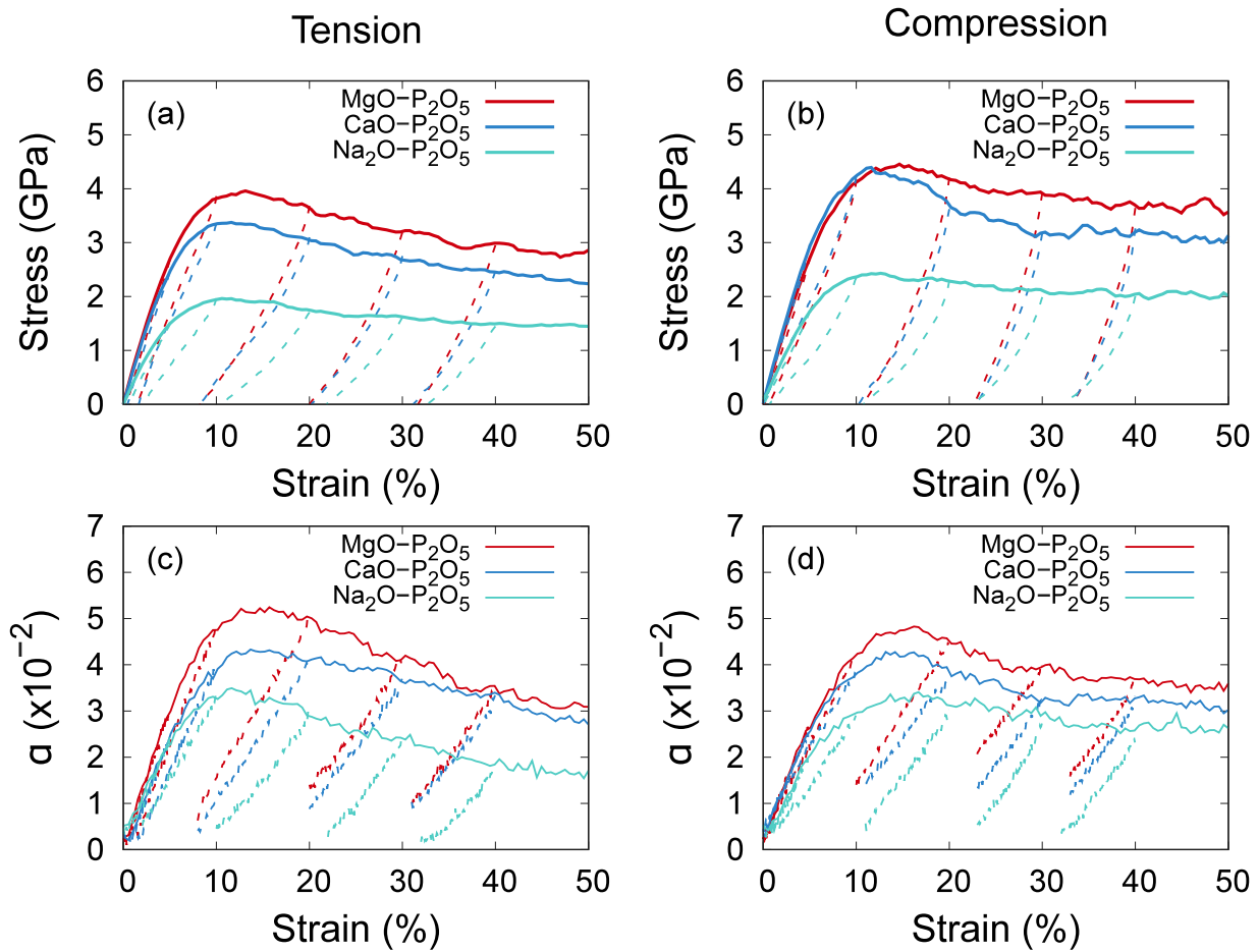
Fig. 2. Stress-strain curves for \text{Na}_2\text{O-P}_2\text{O}_5 , \text{MgO-P}_2\text{O}_5 , and \text{CaO-P}_2\text{O}_5 in (a) tension and (b) compression during the loading from 0% to 50% (solid lines) and unloading from 2.5%, 5%, 10%, 20%, 30%, and 40%. (c and d) show the anisotropy index as a function of the strain during loading and unloading for \text{Na}_2\text{O-P}_2\text{O}_5 , \text{MgO-P}_2\text{O}_5 , and \text{CaO-P}_2\text{O}_5 glasses for both tension and compression, respectively. The strain rate is 5.0 \times 10^8 \text{ s}^{-1} at a constant temperature of 300 K.
