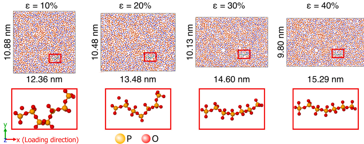
Fig. 7. Top row snapshots at different strains during tensile deformation test (red: O atoms, orange: P atoms, and blue: Na) of \text{Na}_2\text{O}-\text{P}_2\text{O}_5 glass and a single chain is highlighted in green in the red box. The bottom row shows a zoomed-in snapshot of the chain highlighted in the top row, and it orients to be aligned with the deformation axis.
