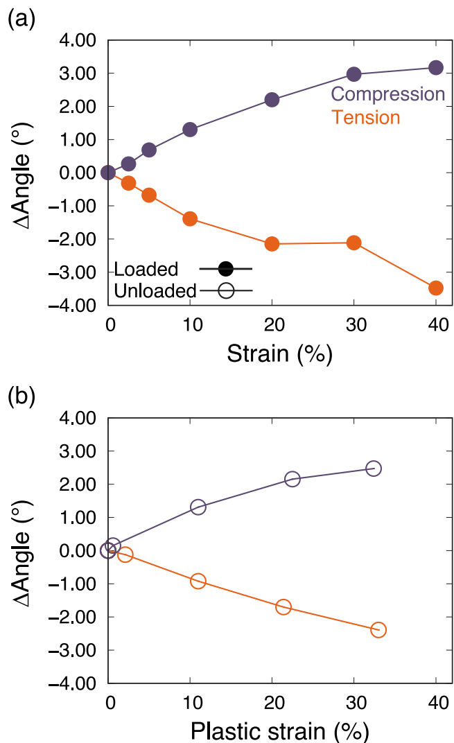
Fig. 6. The difference between the mean chains end-to-end vectors angle in the loaded (a) or unloaded (b) glasses in tension or compression and the pristine Na 2 O-P 2 O 5 glass. The \Delta\text{Angle} = \text{Angle}_{L/U} - \text{Angle}_p , where \text{Angle}_{L/U} is the mean angle between the chain end-to-end vectors and the loading axis in the loaded/unloaded sample and \text{Angle}_p is the mean angle between the chain end-to-end vectors and the loading axis in the pristine glass. For the loaded sample (a), the mean angle difference is plotted as a function of the maximum strain before unloading. The mean angle difference is plotted for the unloaded samples as a function of the remaining plastic strain after unloading to zero stress. The orange color is for tensile deformation, and the violet color is for compression. Closed dots denote loaded samples, and open dots stand for unloaded samples. The lines in both figures are guides for the eyes.
